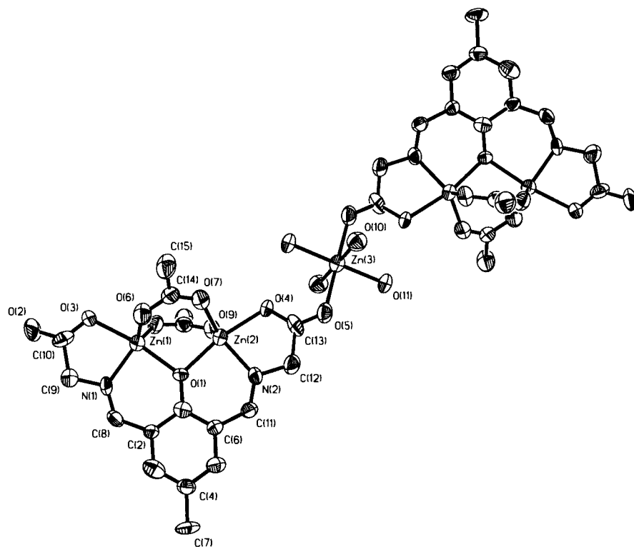
Fig. 4 View of [\{Zn_2L^2(CH_3CO_2)_2\}_2Zn(H_2O)_4] 2 with the atom numbering scheme.
